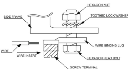
Figure 3. Example of acceptable ground connection
